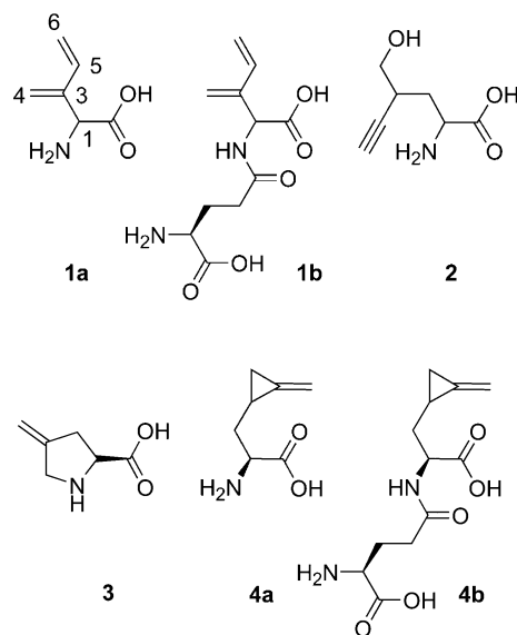
Figure 1. Natural unsaturated \alpha -amino acids.
