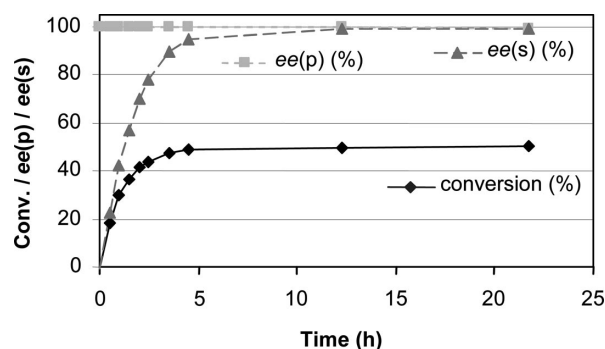
Figure 2. Resolution of 25 by P. putida L-aminopeptidase.
